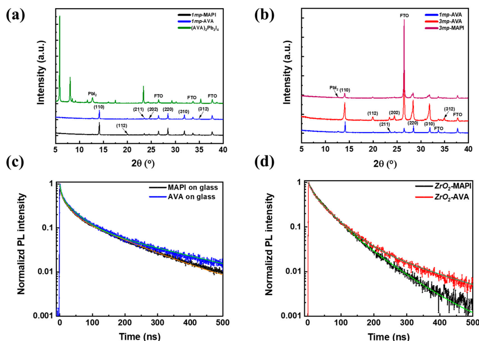
Figure 2. (a) XRD patterns of MAPI, AVA-MAPI, and (\text{AVA})_2\text{PbI}_4 perovskite layers deposited on the 1mp substrate. (b) XRD patterns of 3mp -MAPI and AVA-MAPI layers deposited on 1mp and 3mp substrates. (c) TRPL of 1mp -MAPI and 1mp -AVA layers deposited on glass substrate. (d) TRPL of MAPI and AVA-MAPI layers deposited on mesoporous \text{ZrO}_2/\text{glass} .
