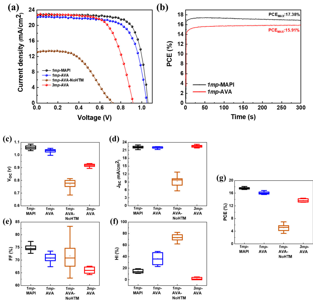
Figure 5. (a) Reverse scan J - V curves of 1mp -MAPI, 1mp -AVA, 1mp -AVA-NoHTM, and 3mp -AVA solar cells. (b) Tracking curves of 1mp -MAPI and 1mp -AVA best cells. (c–g) Statistical analysis of the solar cells J - V curve parameters: (c) V_{oc} , (d) J_{sc} , (e) FF, (f) HI and (g) PCE.
